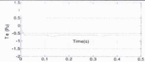
(c) Torque;
