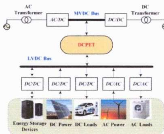
Fig. 1. Typical structure diagram of the dc distribution grid based on DCPET.
