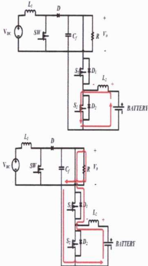
(a) S1 OFF, D2 OFF, S2 ON, D1 OFF (b) S1 ON, D2 OFF, S2 OFF, D1 ON
