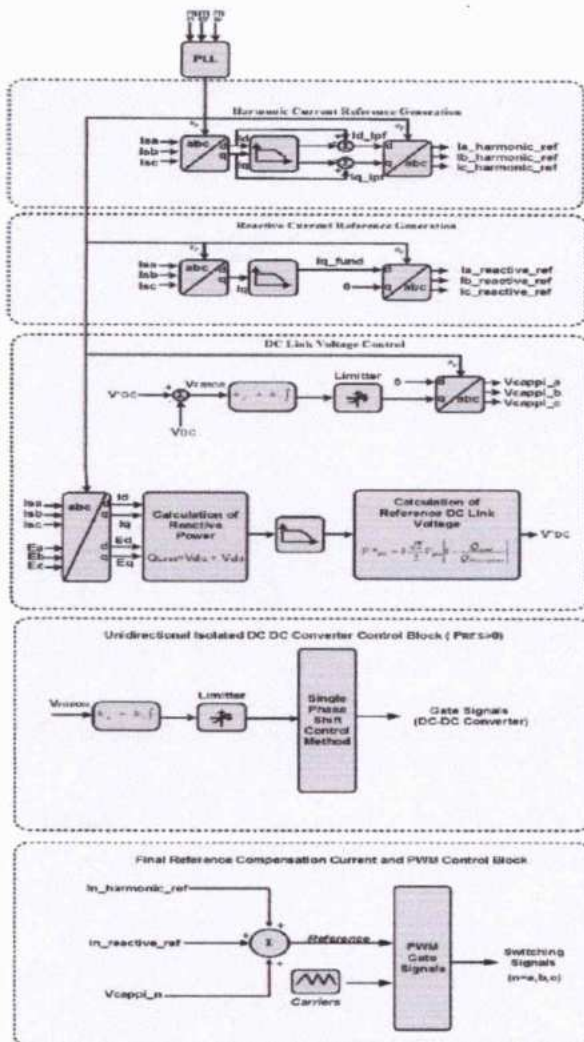
Figure.2. Proposed Controller Block Diagram
