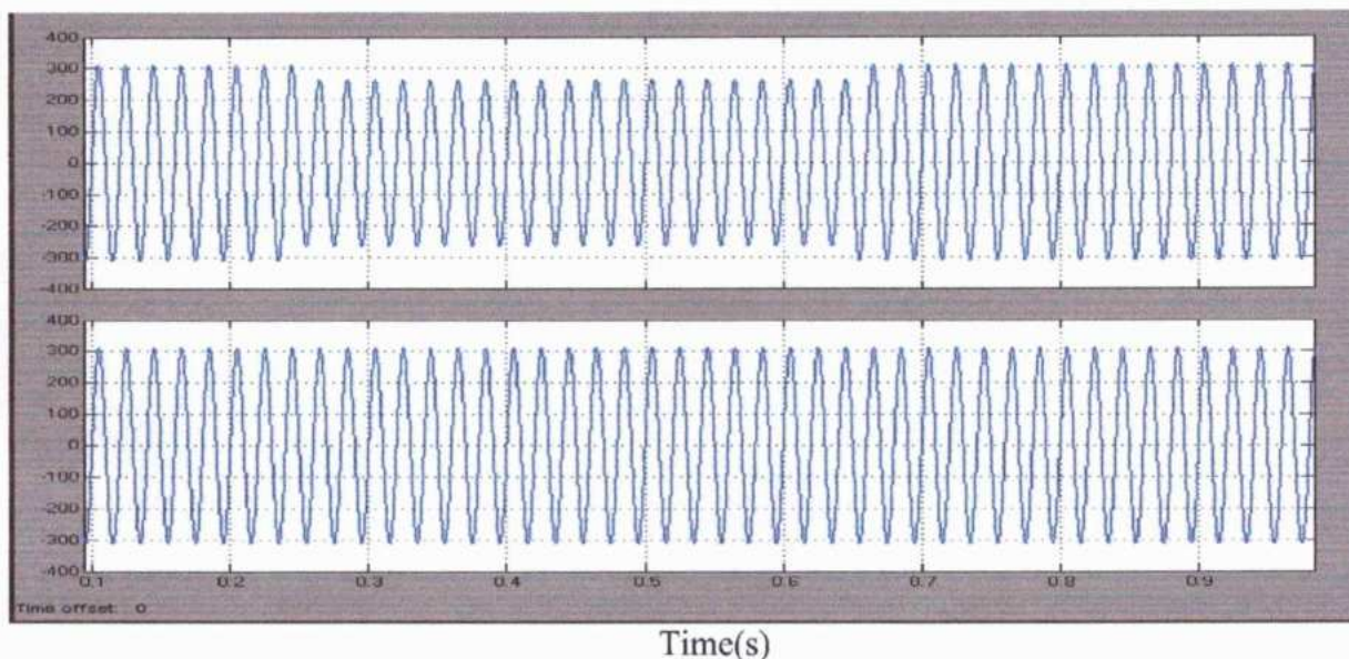
Fig4.3 Performance of the voltage controlled shunt converter with MPPT
