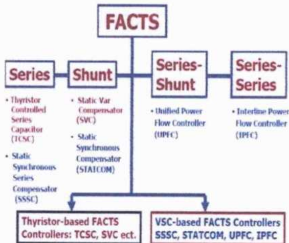
Figure 2 FACTS classification
