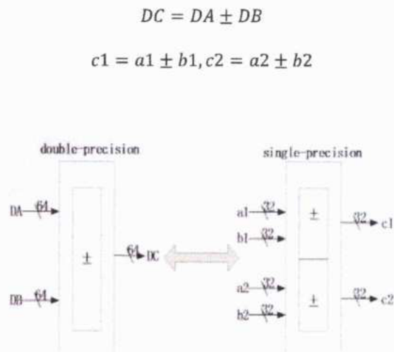
Figure 1.function schematic of multi precision floating point arithmetic
