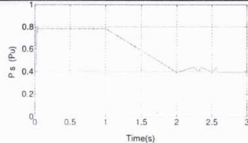
(b) Stator real power;
