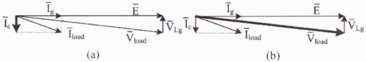
(a) Current-controlled converter (b) Voltage-controlled converter in normal condition.
