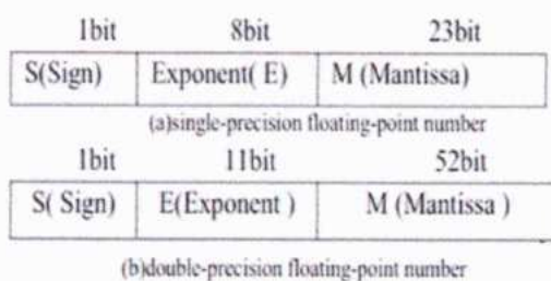
Fig 2 representation of a floating point number
